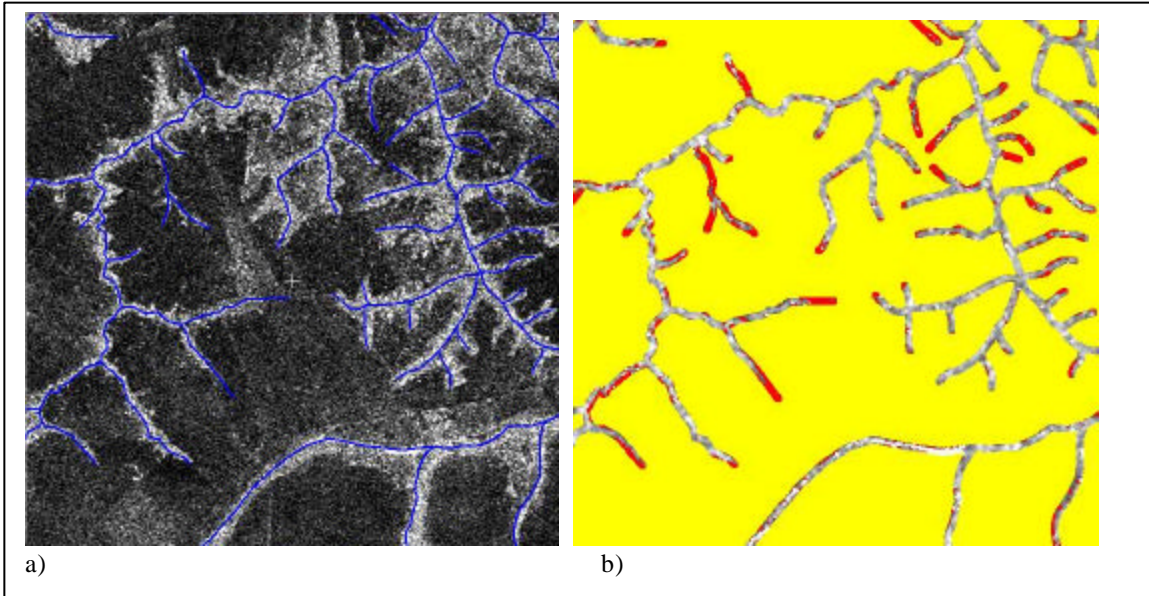
Figure 2: a) 6.4 km \times 6.4 km subset of the original JERS-1 SAR image. b) corresponding subset of the filtered image with the critical areas displayed in red and the areas outside the stream buffer in yellow
