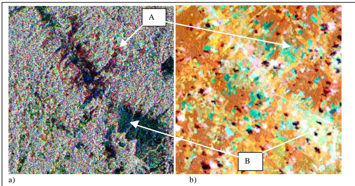
Figure 6: Image subset of a 7.3 km x 7.3 km sector of the road between the towns of Neshuya and Curimaná. a) JERS-1 SAR multi-temporal composition, 30-08-94 in red, 13-11-95 in green and 20-06-96 in blue. b) color-composite Landsat TM image of 22-09-96, bands 4, 5, 3 in red, green and blue.
