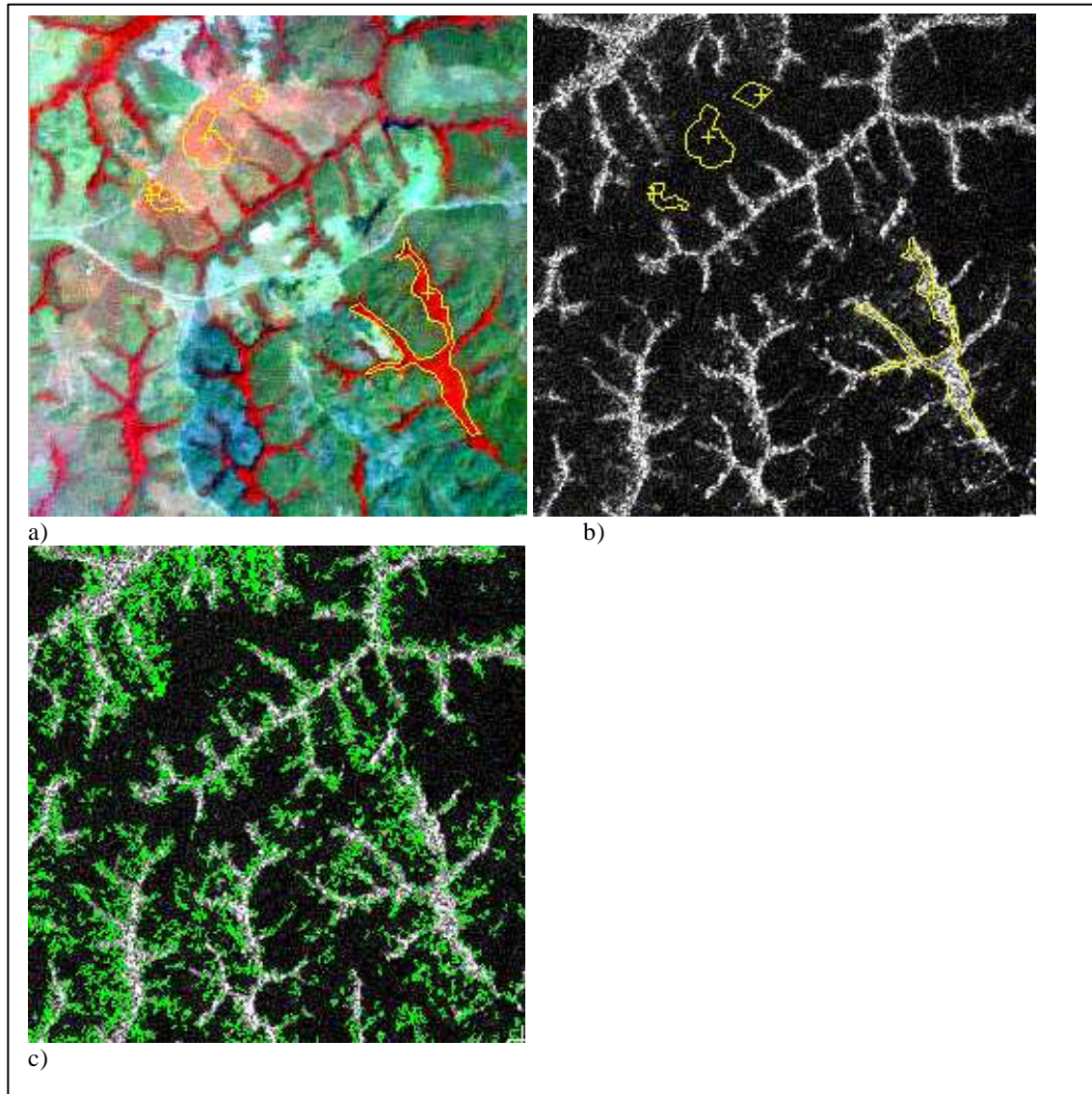
Figure 4: Image subsets (6.25 km \times 6.25 km) in the Puerto López municipality. a) Landsat TM, 09-01-1996, assignment of bands 4, 5 and 3 in the Red, Green and Blue display channels. B) JERS-1 SAR of 21-03-96 c) JERS-1SAR with the areas segmented as scrubland in green
